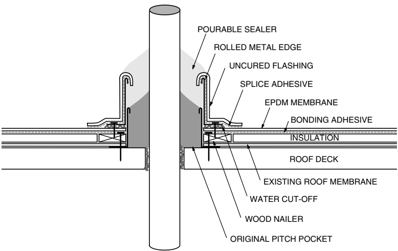
Figure 31b – Reroof
