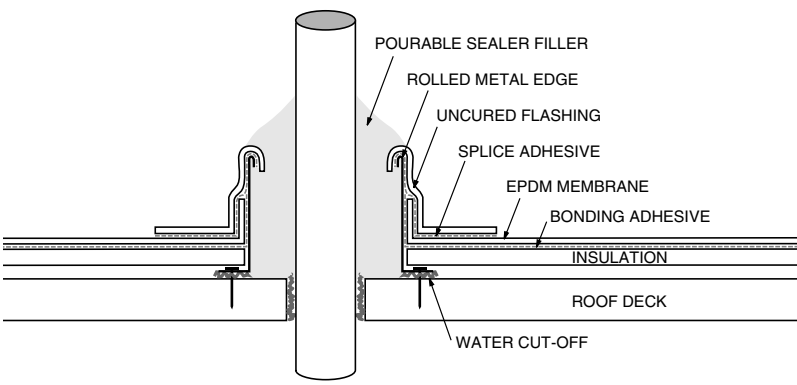
Figure 31b – Reroof
